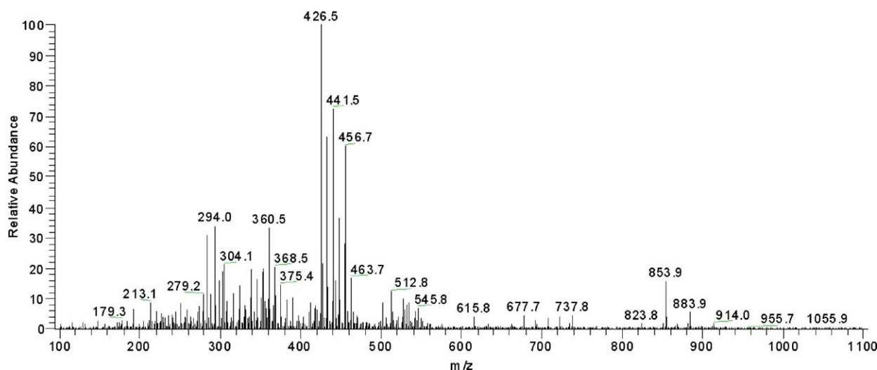
Fig. 7. EIS-MS analysis of oligomannuronate 5 mer. The peak at m/z 914.0 corresponds to the molecular ion peak [\text{M}-1]^{-1} of the 5 mer. The ionic fragments of the 5 mer were also detected.
